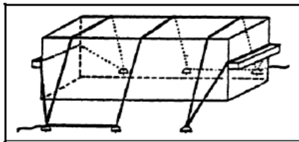
Figure 41 Human Remains Tie-Down Scheme
