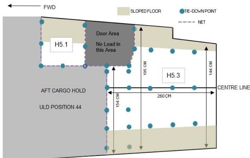
Figure 34 Bulk Hold (inc. ULD Position 44)
