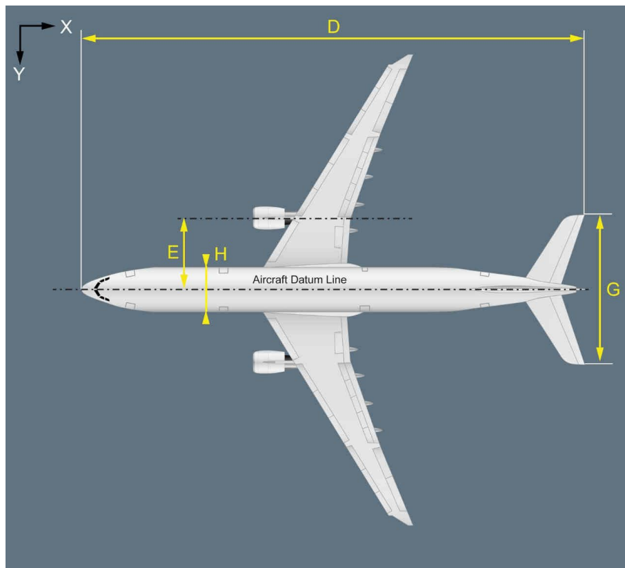
Figure 38 Aircraft Dimensions (top)
