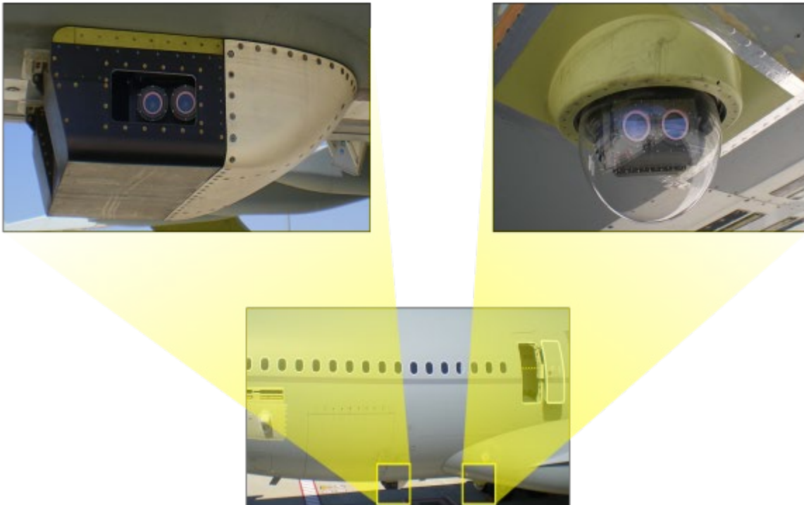
Figure 69 Optional fit
